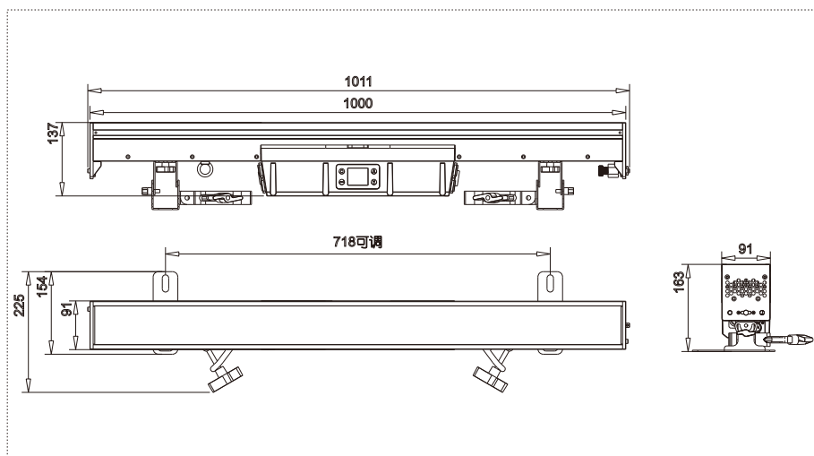
Size-Fig.2(Unit: mm)
