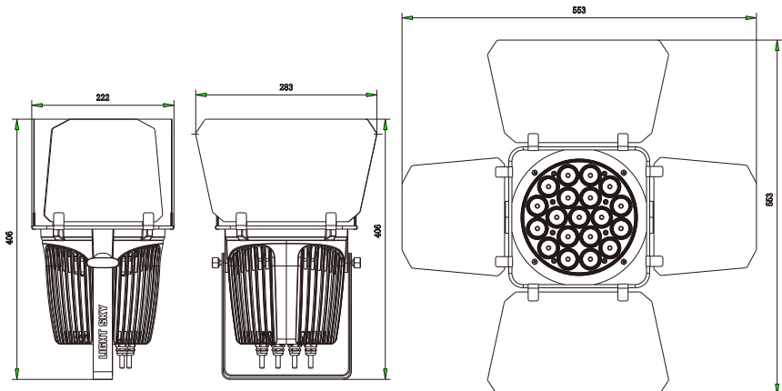
Body Size---Fig 2
