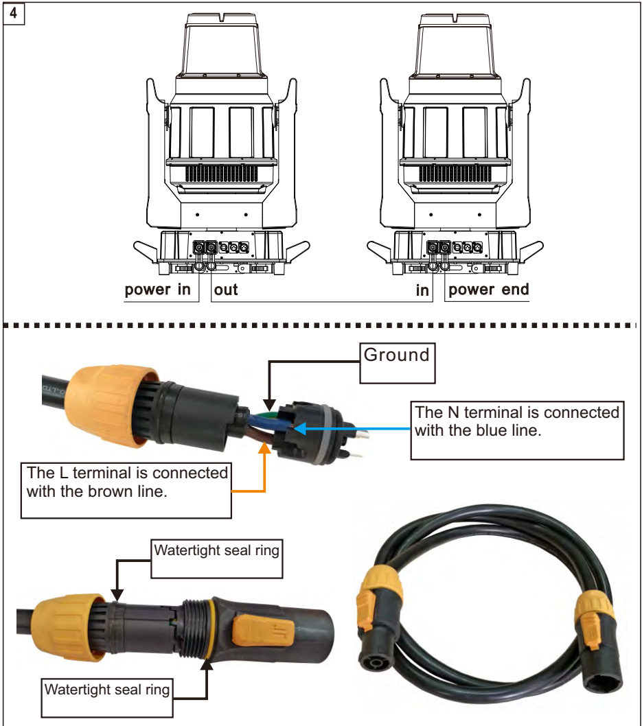
Connecting to the mains supply ---Fig 4
